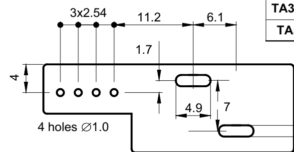
TA37.5A-P..TA50A-P PCB mounting hole layout
